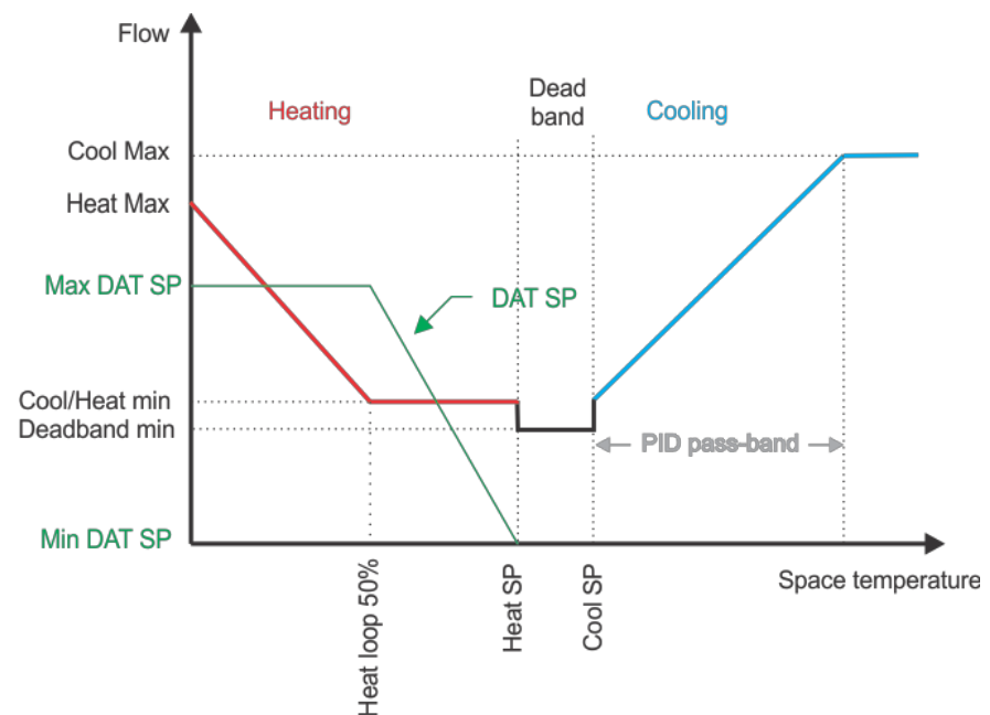
Figure 6.3 – Reheat mode.
