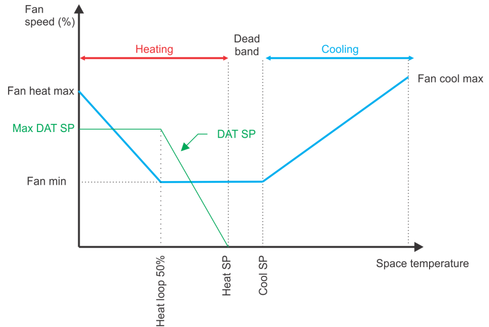
Figure 6.5 – Series fan logic.
