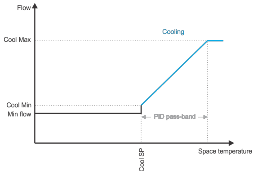
Figure 6.1 – Cool-only mode.
