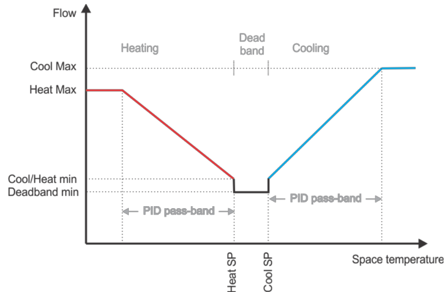
Figure 6.2 – Changeover mode.
