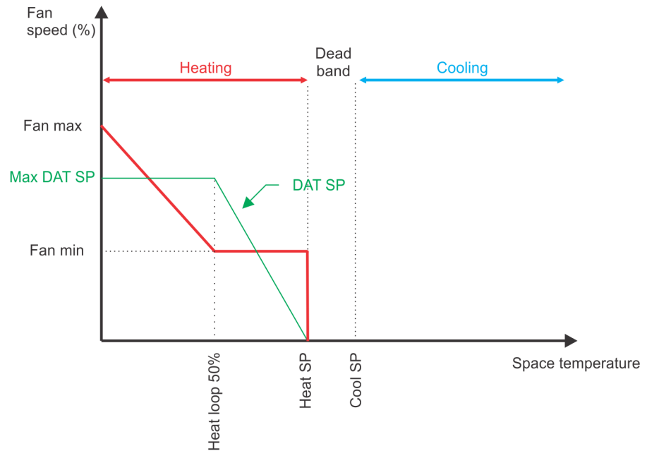
Figure 6.4 – Parallel fan logic.
